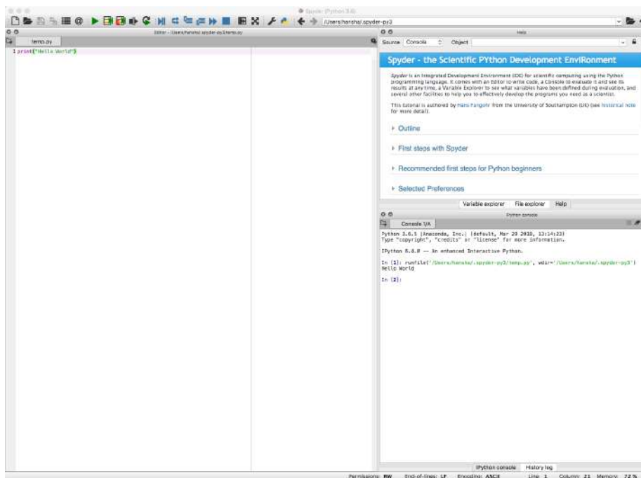
Figure 17.1: Spyder Editor
