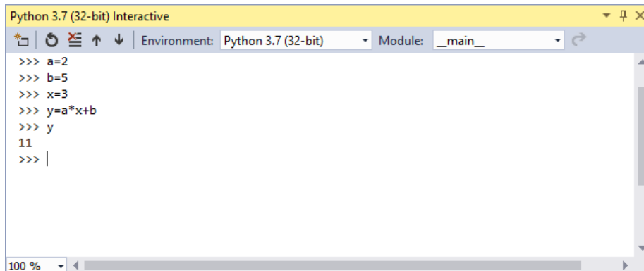
Figure 19.4: Python Interactive
