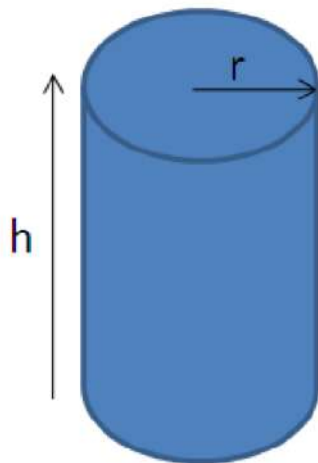
Figure 23.2: cylinder
