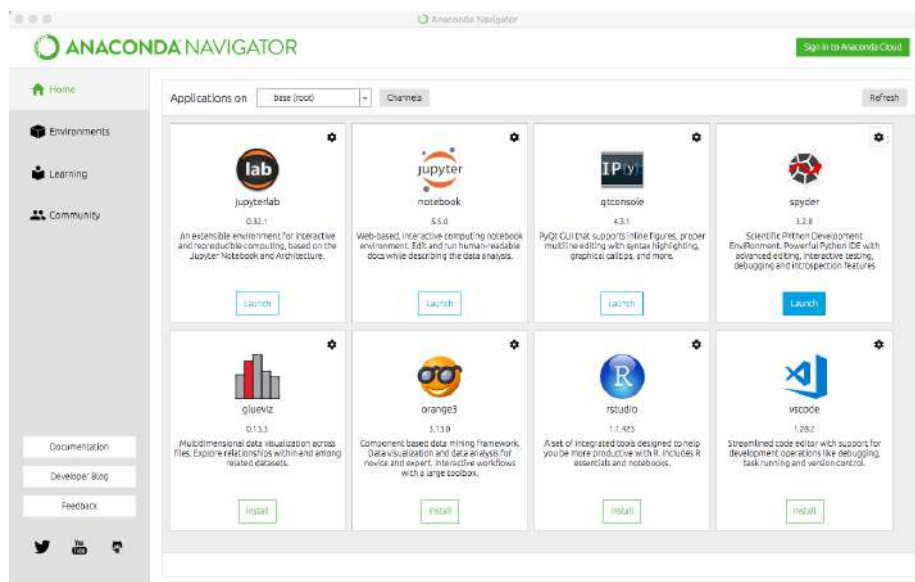
Figure 14.1: Anaconda Navigator
